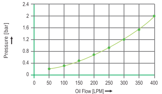
PRESSURE DROP
